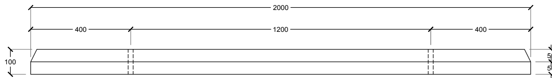
SIDE VIEW
